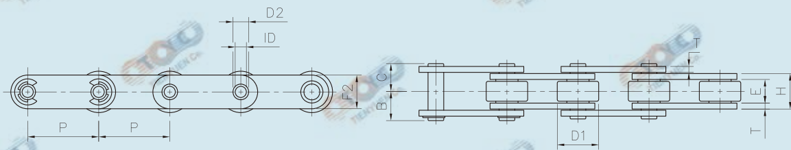
Double Pitch Series with Large Roller
